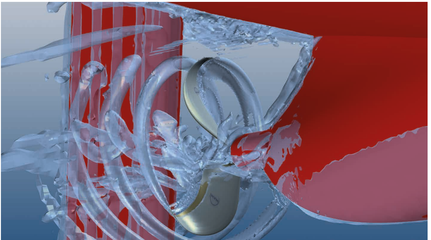
Transient simulation of the self-propulsion of a bulk carrier using the tip modified Kappel Propeller.
