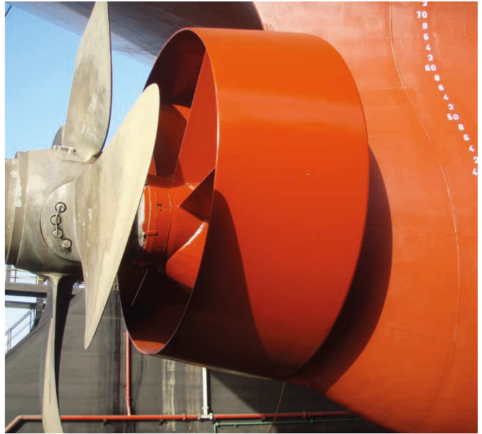
IBMV utilized a STAR-CCM+ digital twin to design the Becker Mewis duct in six weeks, delivering $500k per year per ship in fuel savings.
